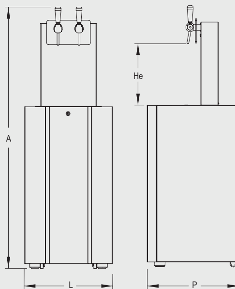
BLUBAR Floorstanding
